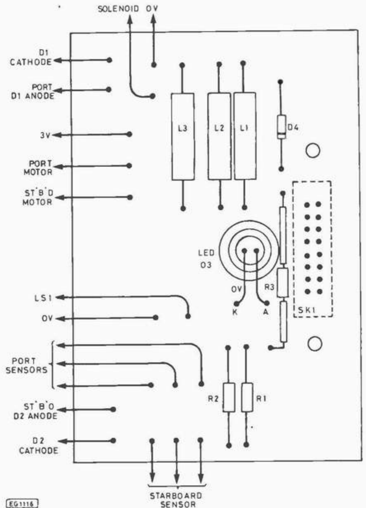
Fig. 10. Component layout
