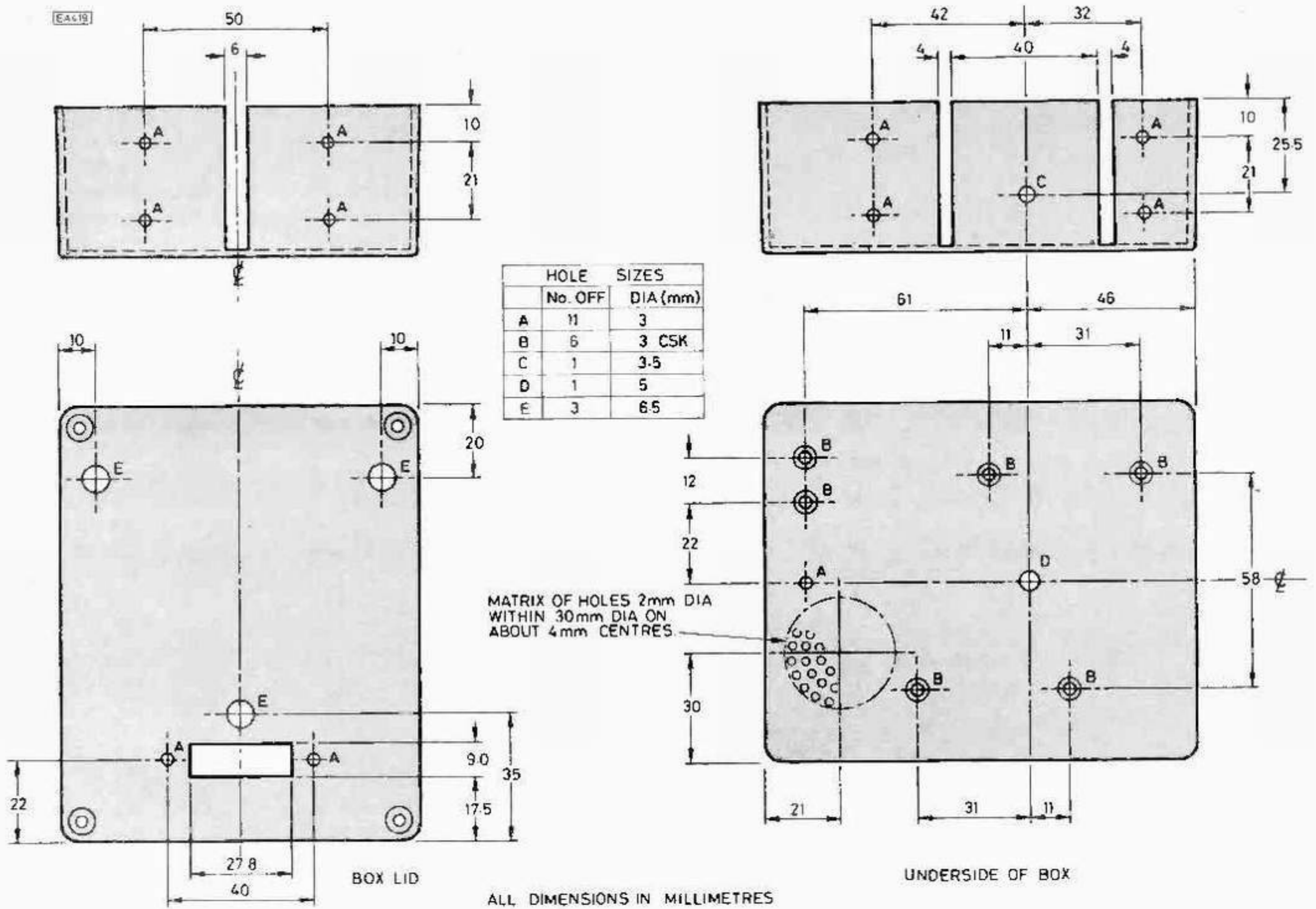
Fig. 1. Cutting and drilling details for Zeaker's chassis
