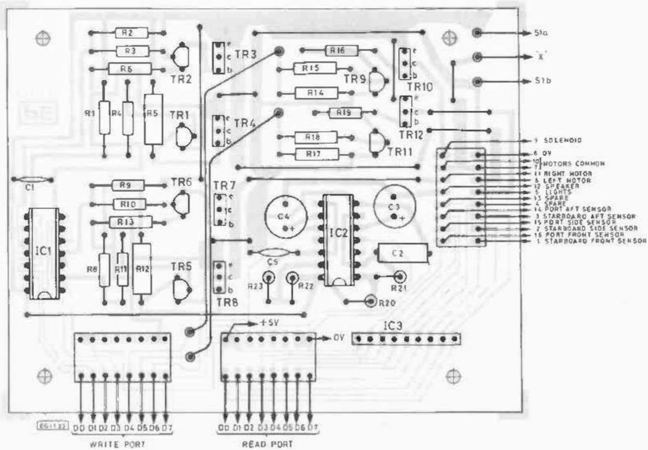
Fig. 3. Component layout
