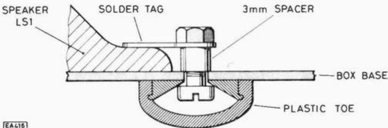
Fig. 8. Toe assembly
