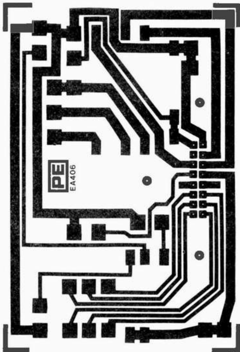
Fig. 9. P.c.b. for vehicle
