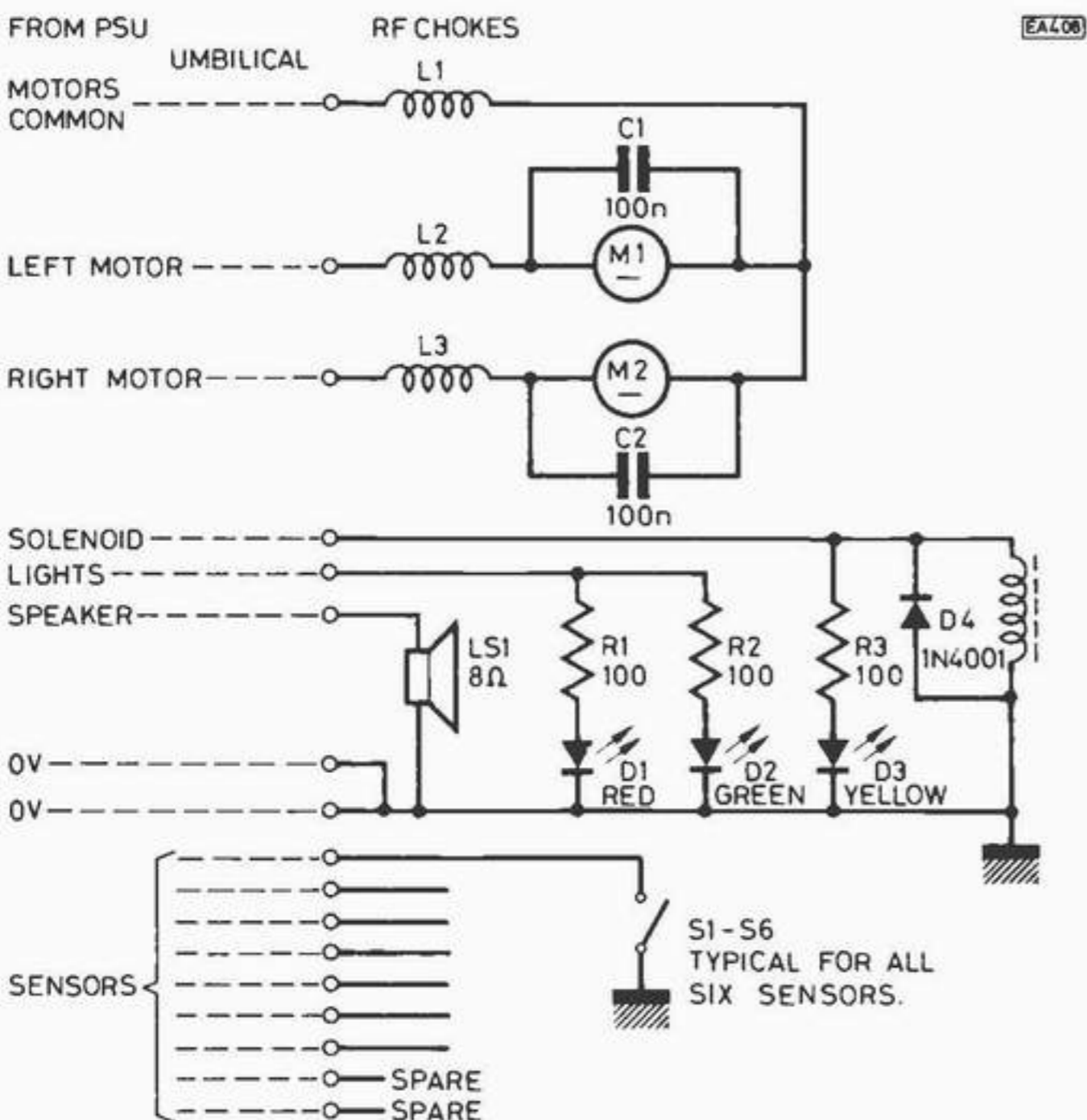
Fig. 13. Wiring diagram for the vehicle
