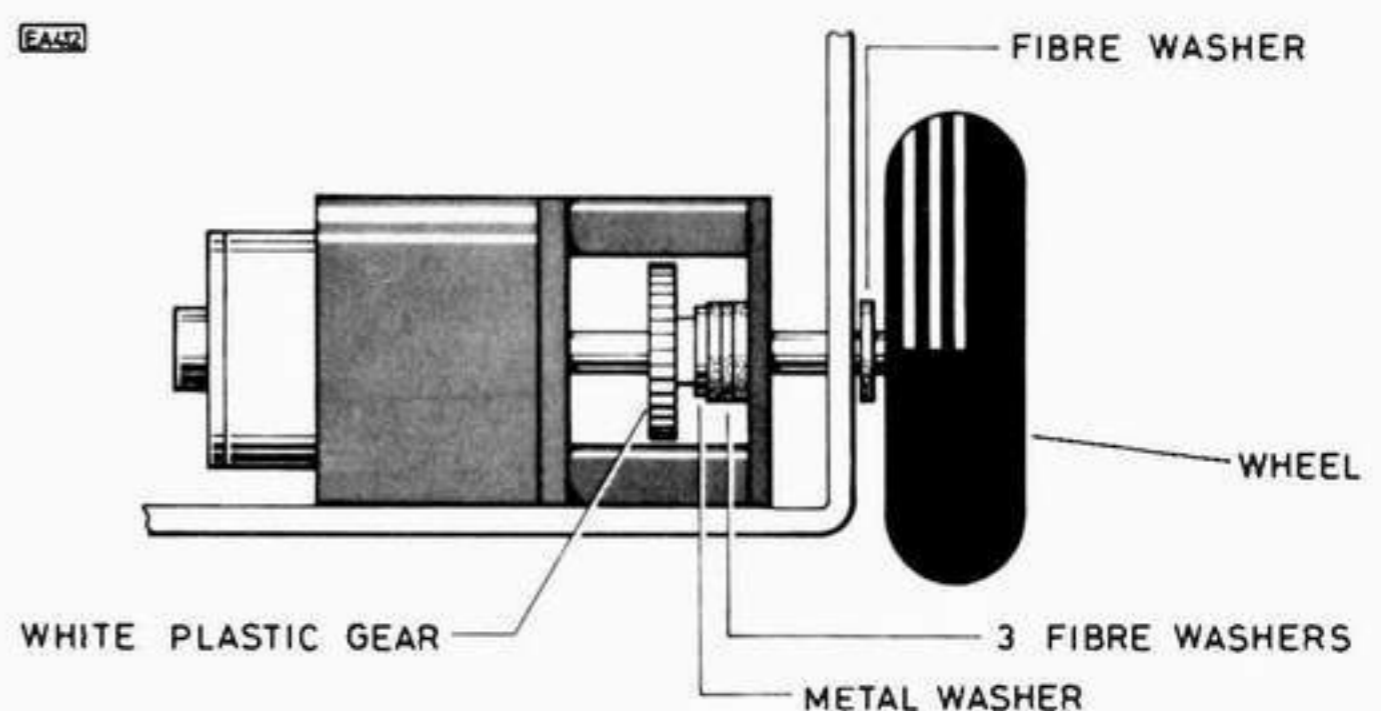
Fig. 6. Motor, gearbox and wheel assembly
