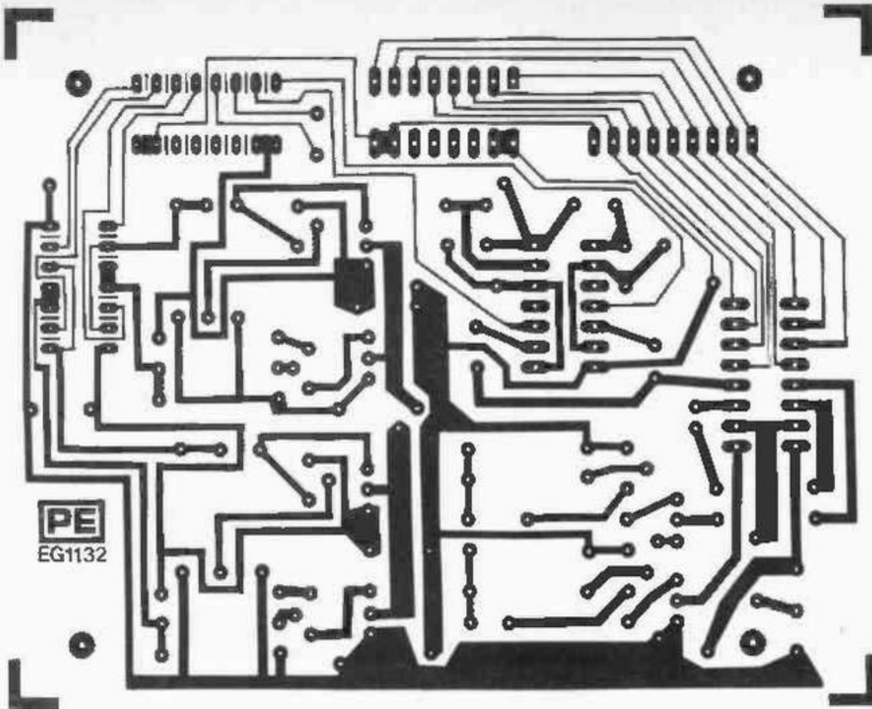
Fig. 2. P.c.b. design
