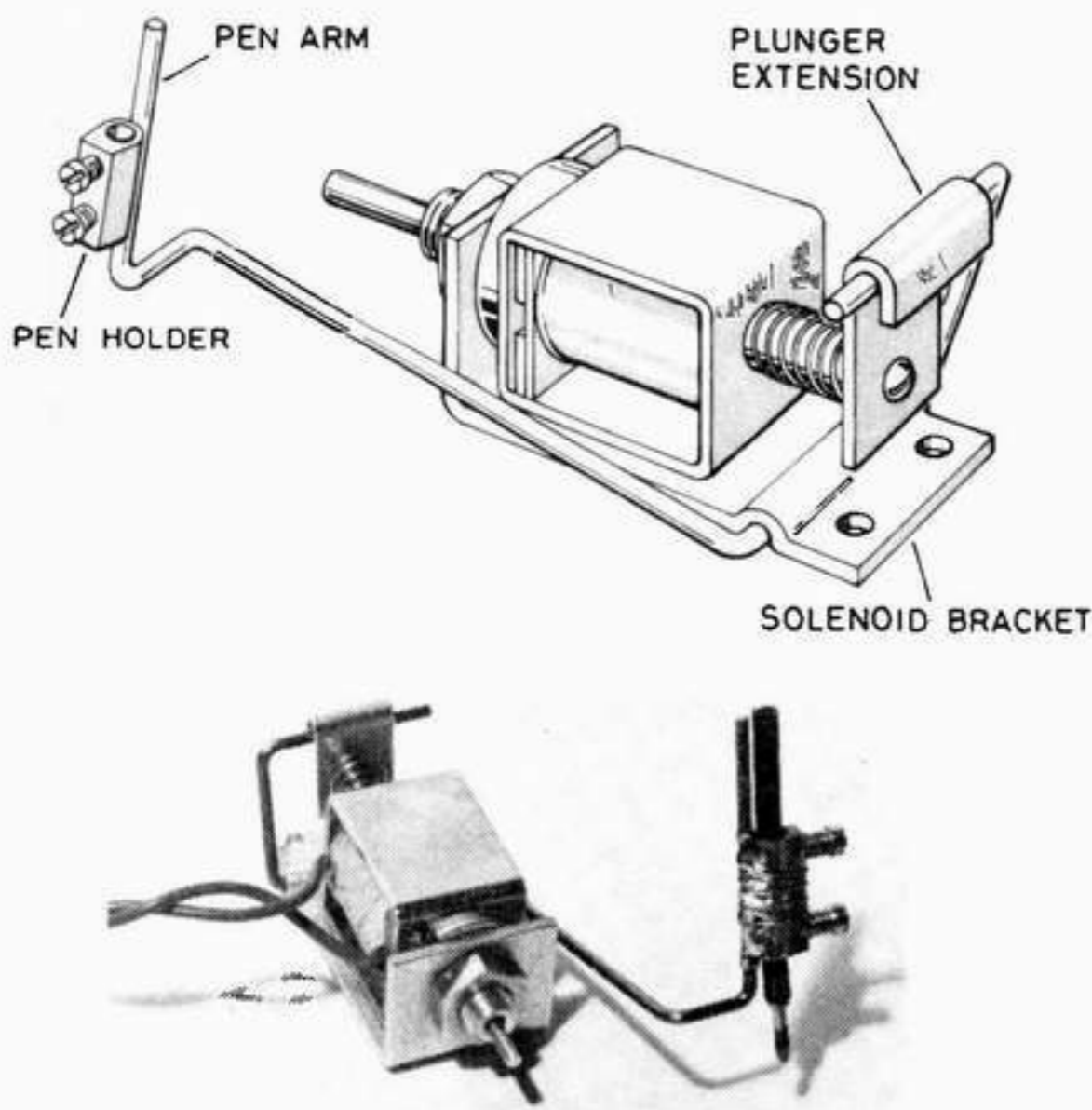
Fig. 4. Solenoid mounting bracket and pen arm. Note the pen arm drawing is full size and can be used as a template for cutting and bending the arm
