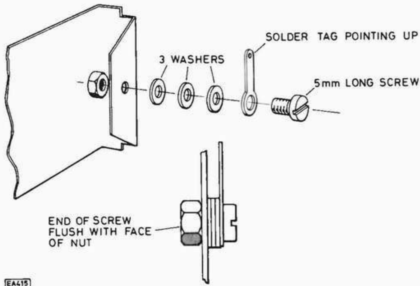
Fig. 3. Method for attaching solder tags to fenders
