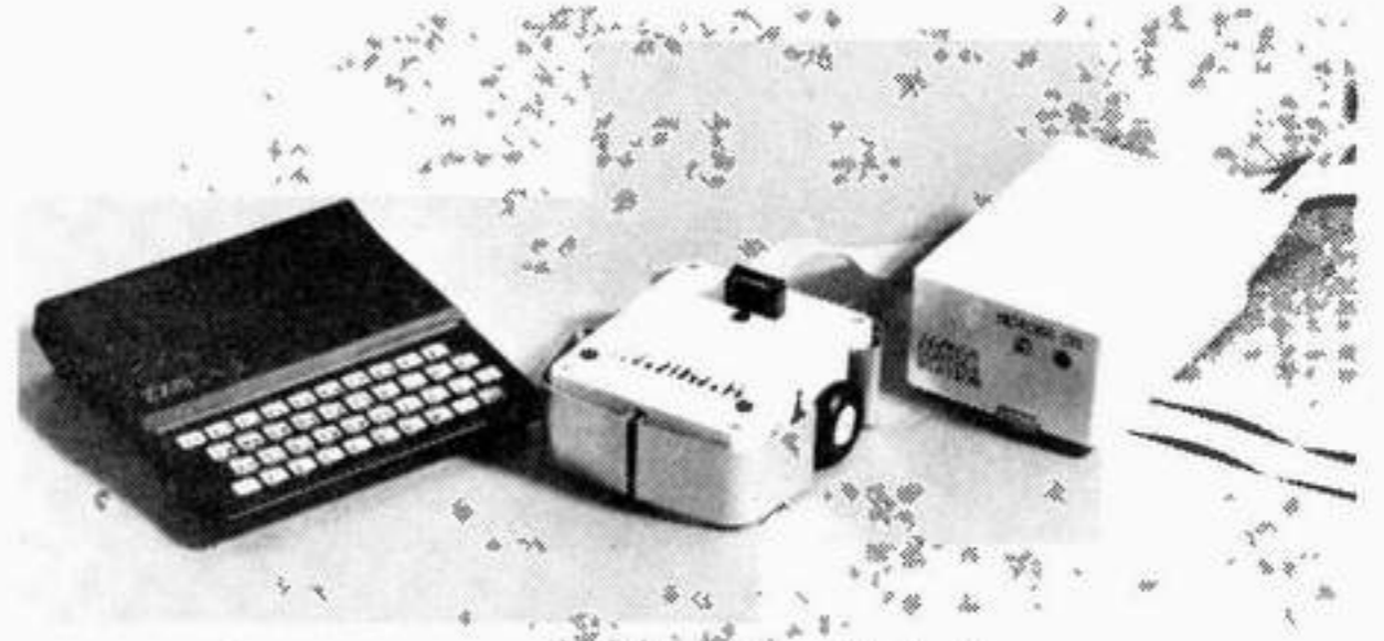
The Zeaker Vehicle together with its Control Station and a ZX-81
