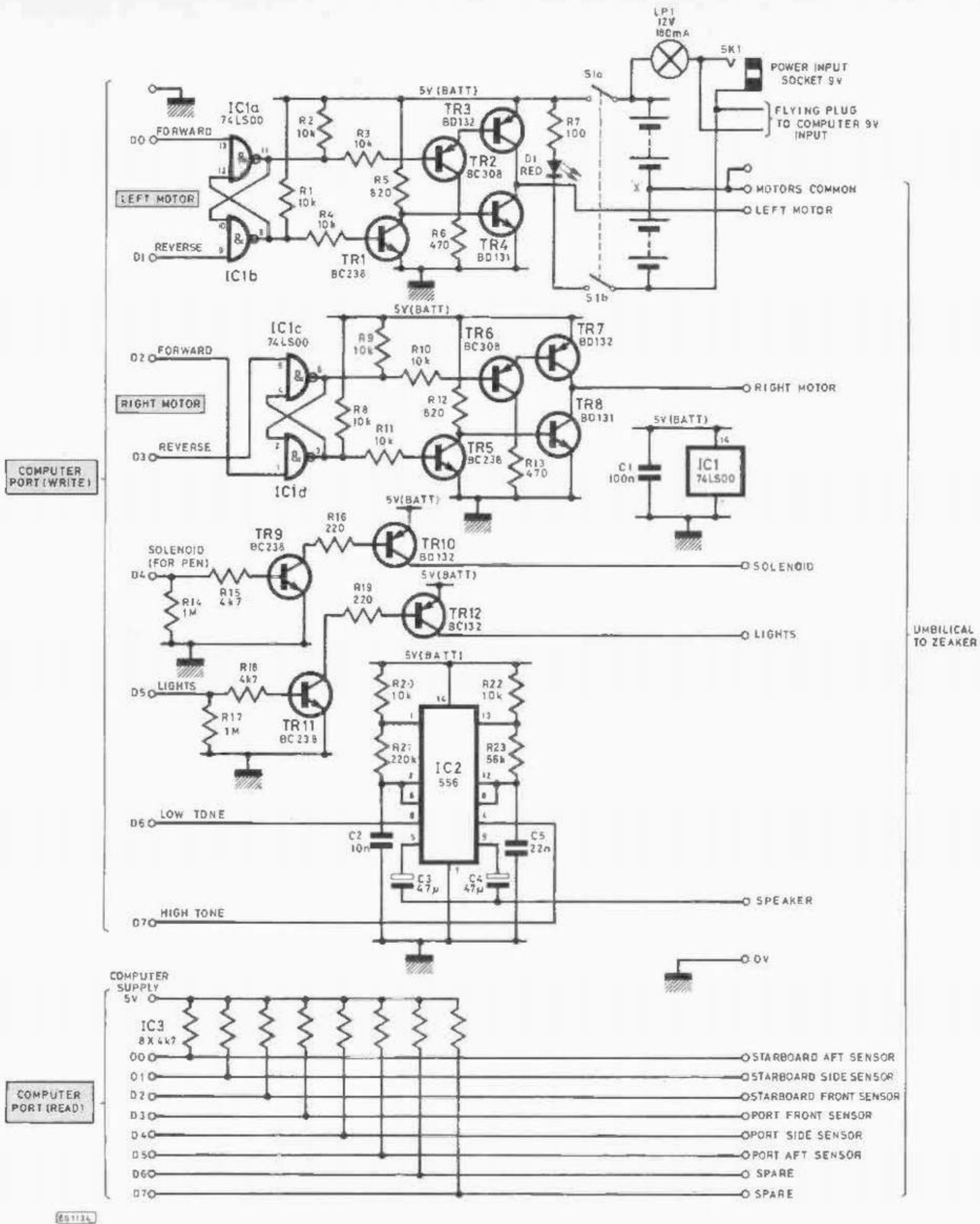
Fig. 1. Circuit diagram of the Control Station
