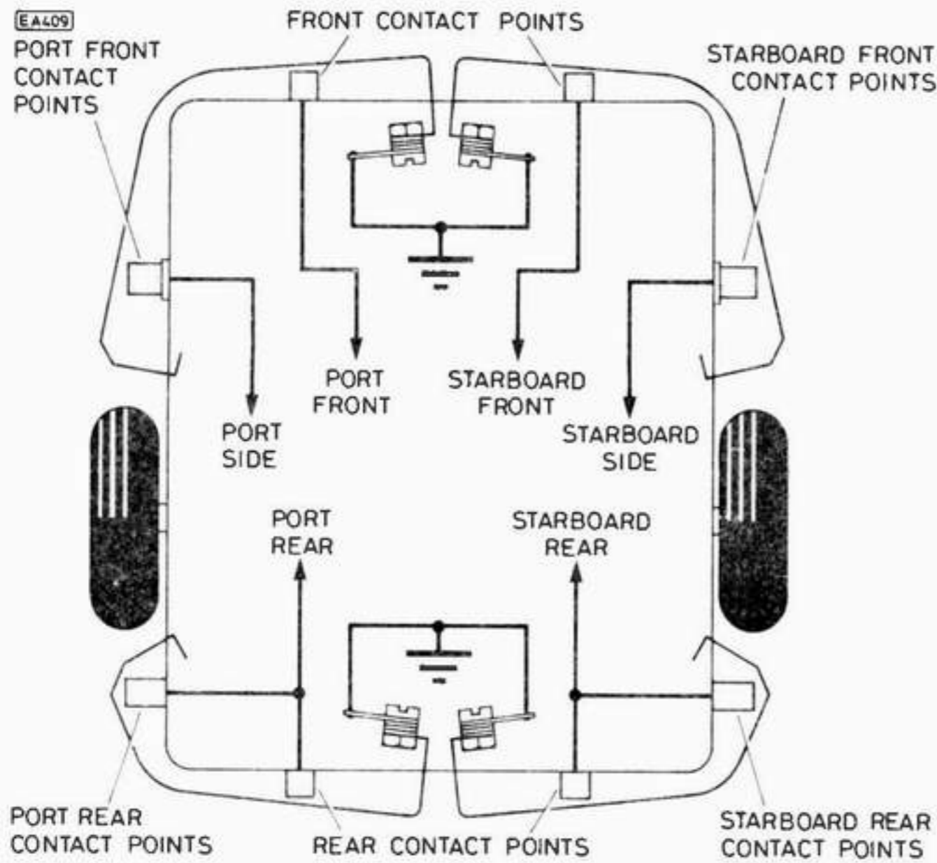
Fig. 11. Location of Zeaker's tactile sensors
