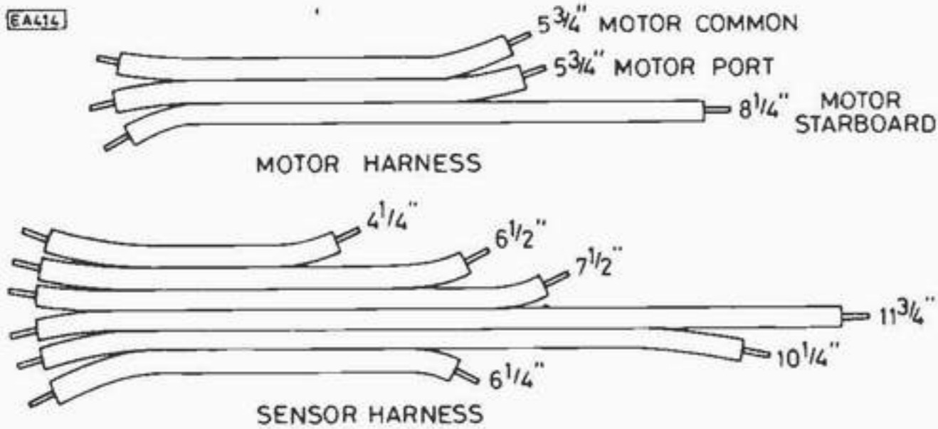
Fig. 12. Motor and Sensor harnesses
